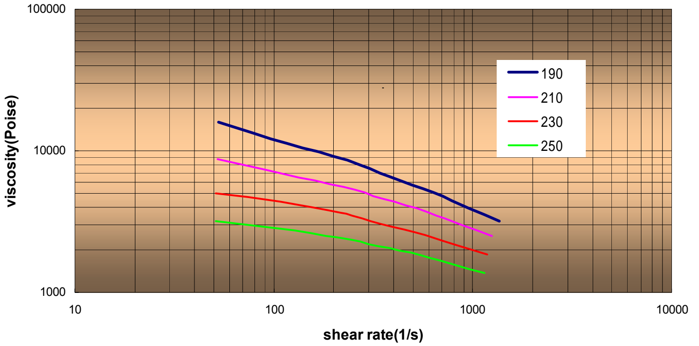
EV4405V Melt Viscosity Curve
